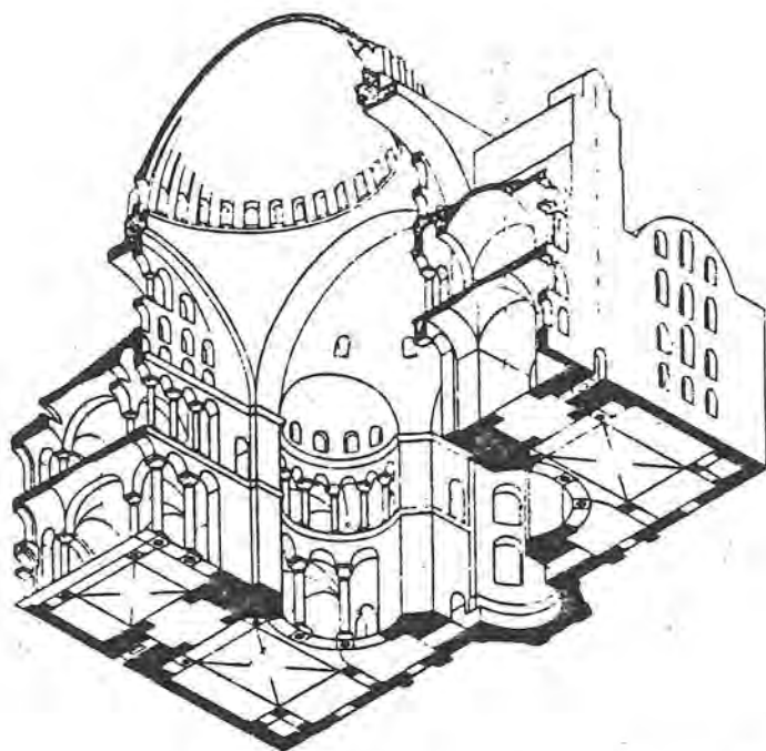
Plate 5. Hagia Sophia, Constantinople, (532-537 A.D.). Analytical half-section. (W. MacDonald, Early Christian and Byzantine Architecture , plate 55.)
